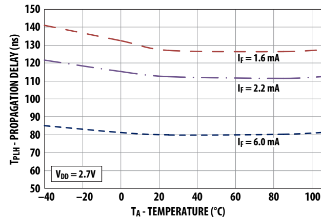
Figure 14: Propagation Delay, t_{PLH} vs. Temperature
