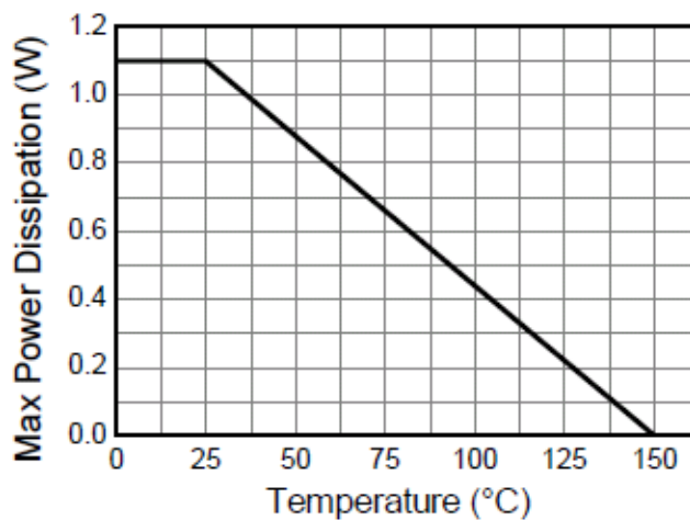
Derating Curve
