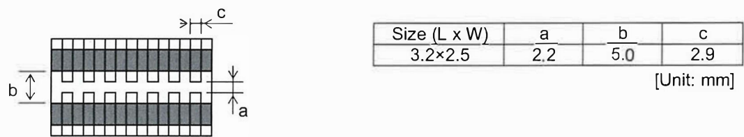
Fig. 2: Board of Adhesive Force of Terminal Electrodes, Vibration, and Thermal Shock Tests
