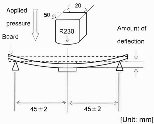
Fig. 4: Bending Strength Test Method
