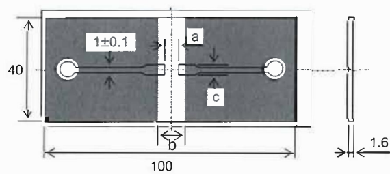
Fig. 3: Board for Bending Strength Test
