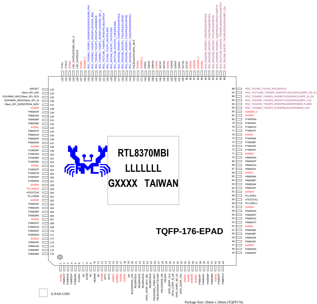
Figure 7. Pin Assignments
