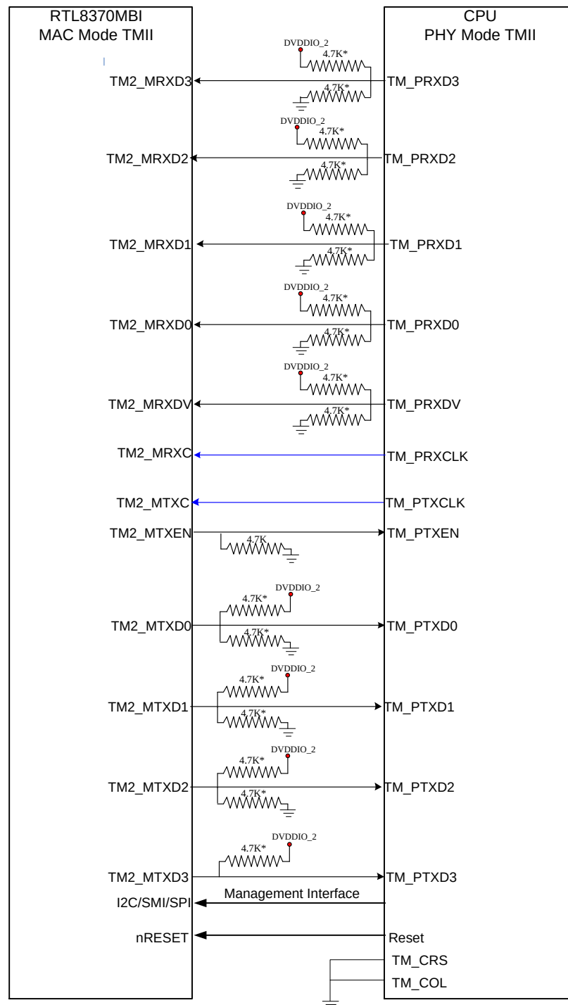
Figure 40. Signal Diagram of TMII MAC Mode of the Extension GMAC2
