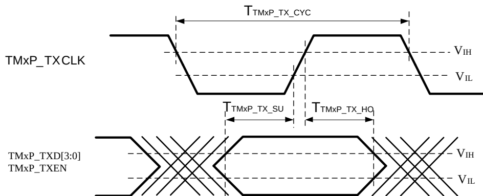
Figure 66. TMII PHY Mode Input Timing
