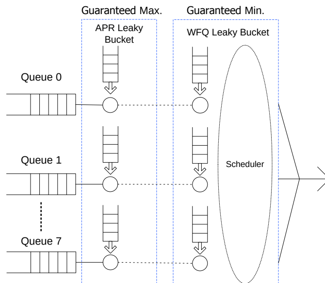
Figure 10. RTL8370MBI MAX-MIN Scheduling Diagram
