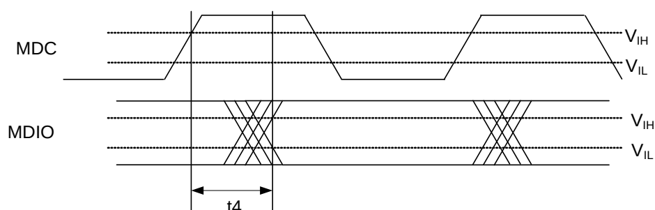
Figure 53. MDIO Sourced by Slave (RTL8370MBI)
