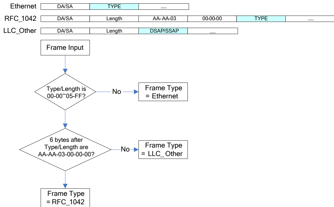
Figure 9. Protocol-Based VLAN Frame Format and Flow Chart
