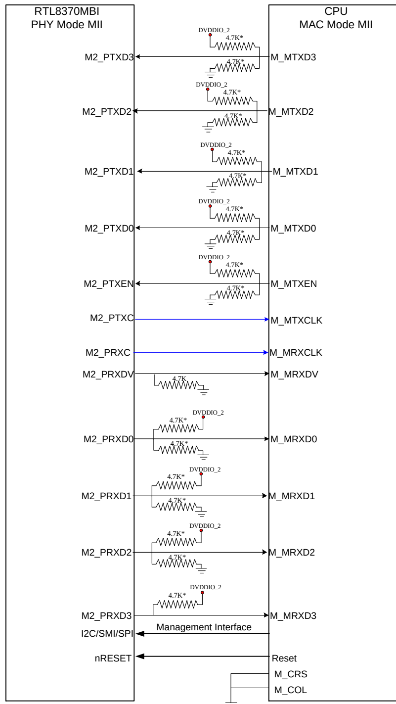
Figure 35. Signal Diagram of MII PHY Mode of the Extension GMAC2
