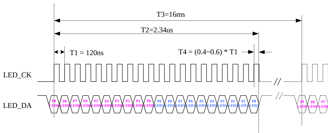
Figure 17. RTL8370MBI Serial Shift LED; Per-Port Two Single-Color LED
