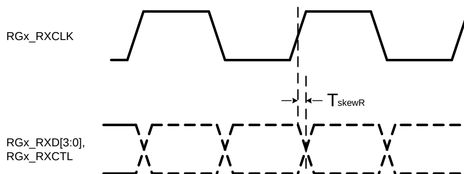
Figure 58. RGMII Input Timing Characteristics (RGx_RXCLK_DELAY=2ns)
