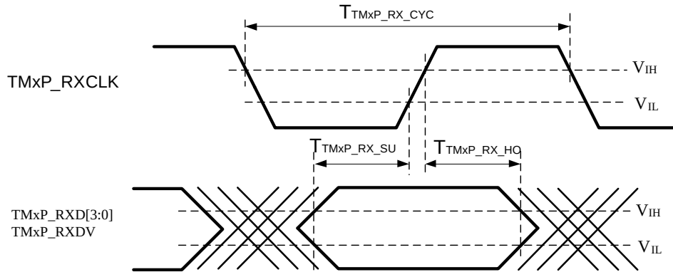
Figure 65. TMII PHY Mode Output Timing
