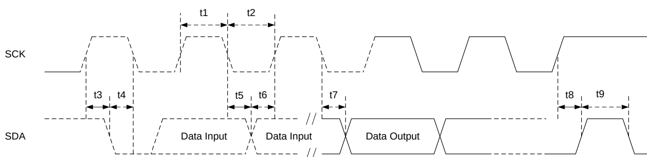
Figure 51. I2C-Like Slave Mode for External CPU Access Interface Timing Characteristics
