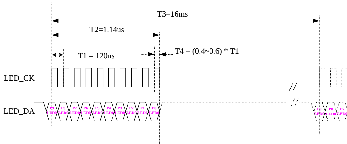
Figure 18. RTL8370MBI Serial Shift LED; Per-Port One Single-Color LED
