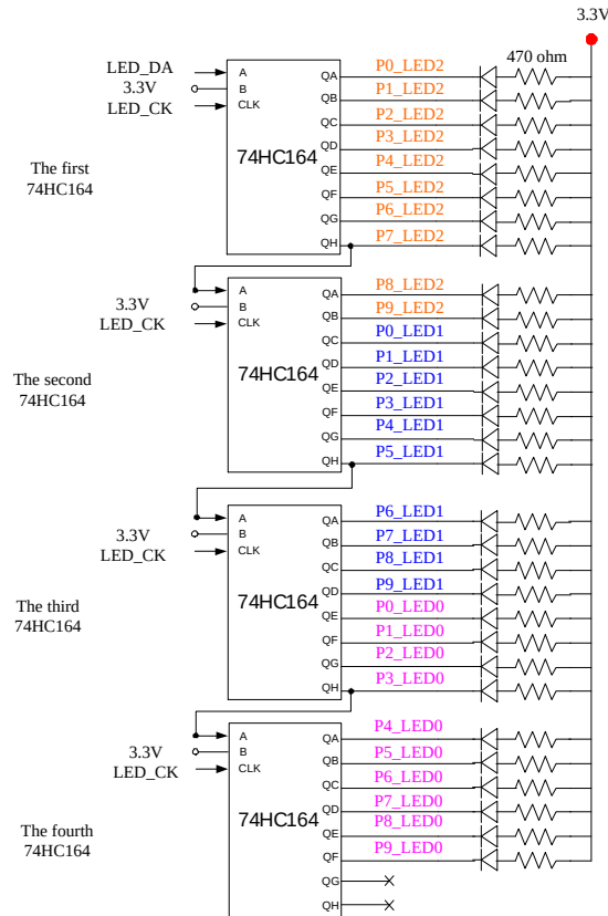
Figure 14. RTL8370MBI+74HC164 Serial LED Connection Diagram (Per-Port Three Single-Color LED)
