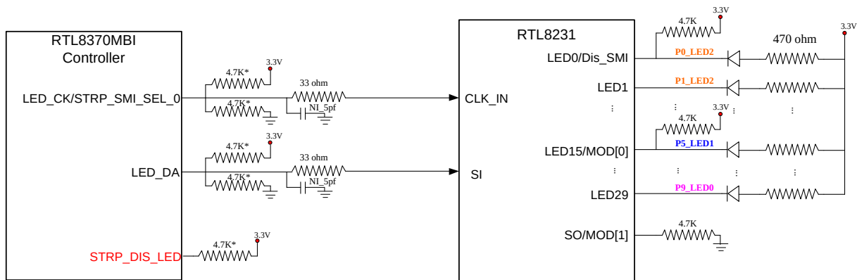
Figure 16. RTL8370MBI+RTL8231 Serial LED Connection Diagram (Per-Port Three Single-Color LED)
