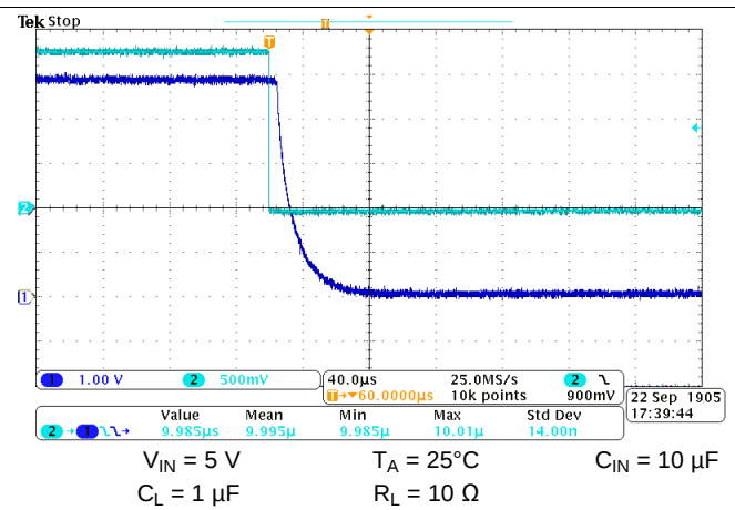
Figure 68. Turn-off Response
