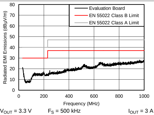
Figure 31. LM43603PWPEVM Radiated EMI Curve
