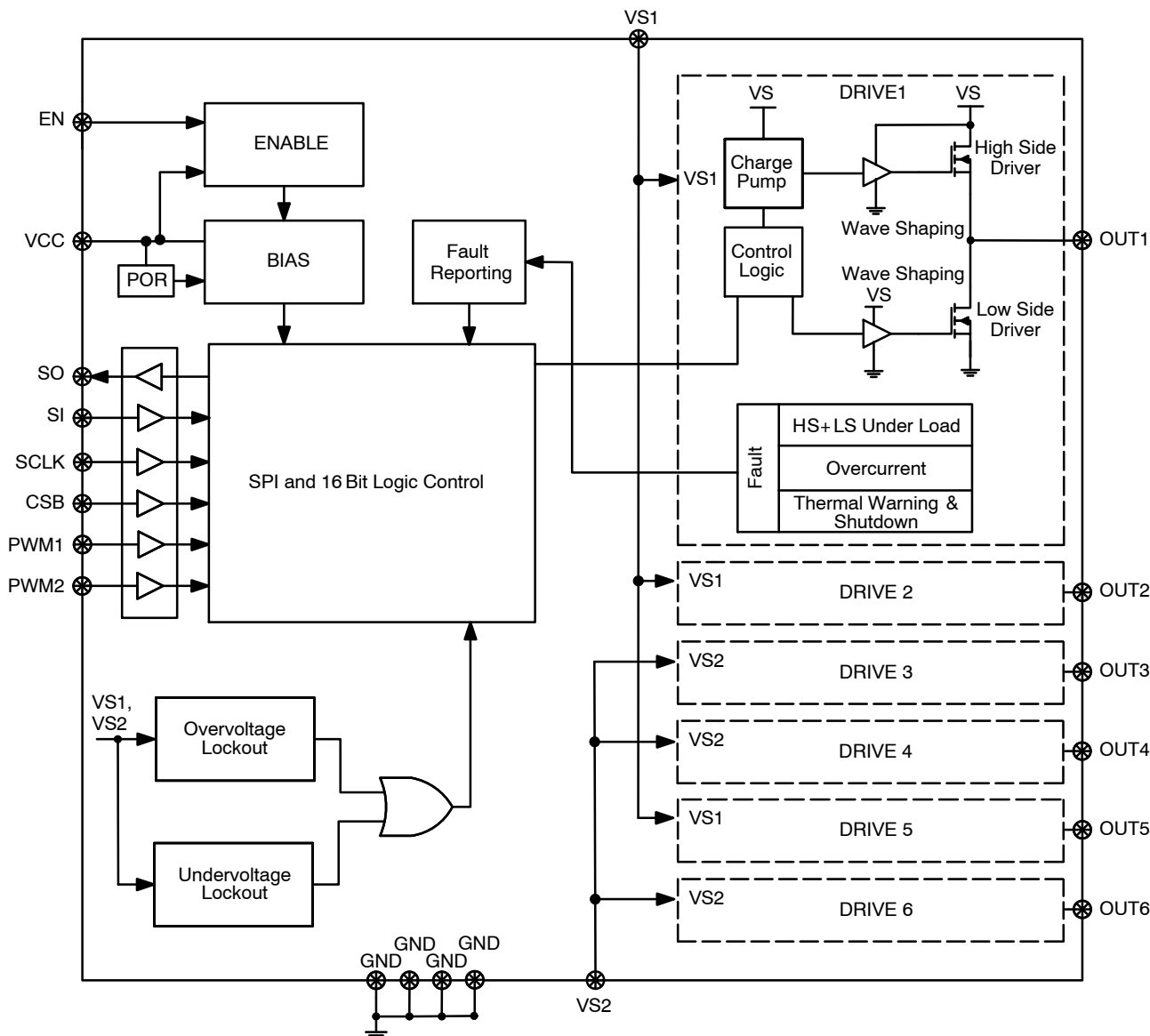
Figure 2. Block Diagram
