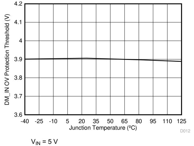
图 6-12. DM_IN Overvoltage Protection Threshold vs Temperature
