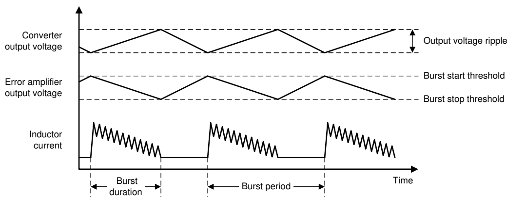
图 13. Pulse-Frequency Modulation
