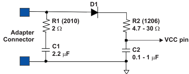
Figure 12. Input Filter
