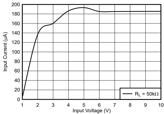
图 5-5. Input Current vs Input Voltage ( R_L = 50k\Omega )
