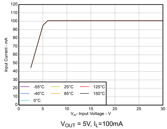
图 5-8. Input Current vs Input Voltage ( R_L = 50 \Omega ) (New Chip) V_{OUT} = 5V, I_L = 100mA
