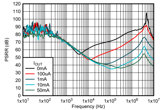
图 5-56. Ripple Rejection vs Frequency (Legacy Chip)
