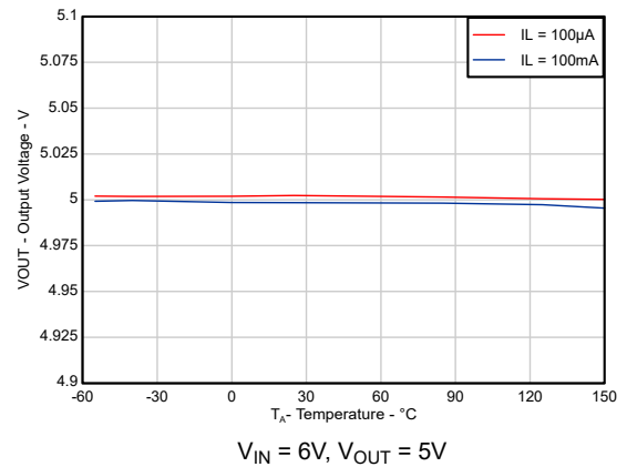
图 5-10. Output Voltage vs Temperature (New Chip) V_{IN} = 6V, V_{OUT} = 5V
