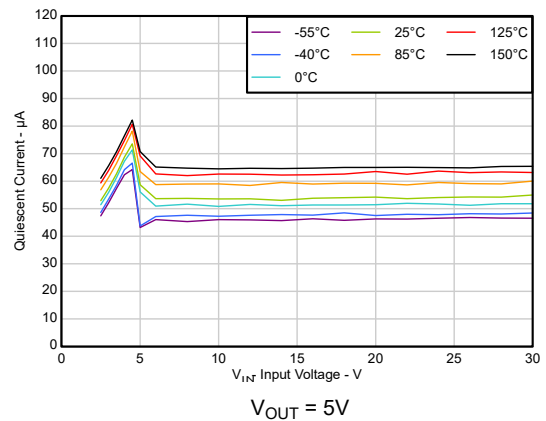
图 5-12. Quiescent Current vs Input Voltage ( I_L = 0 ) (New Chip) V_{OUT} = 5V
