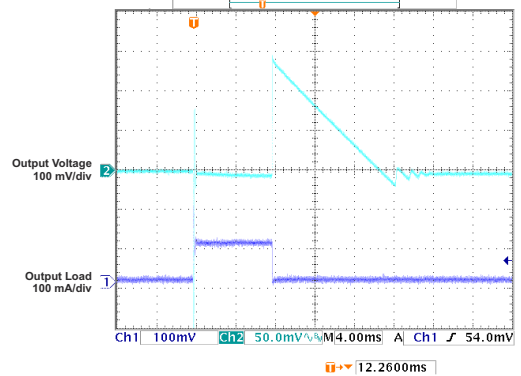
图 5-47. Load Transient Response vs Time ( V_{OUT} = 5V, C_L = 10\mu F ) (Legacy Chip)
