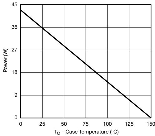
Power, Junction-to-Case
