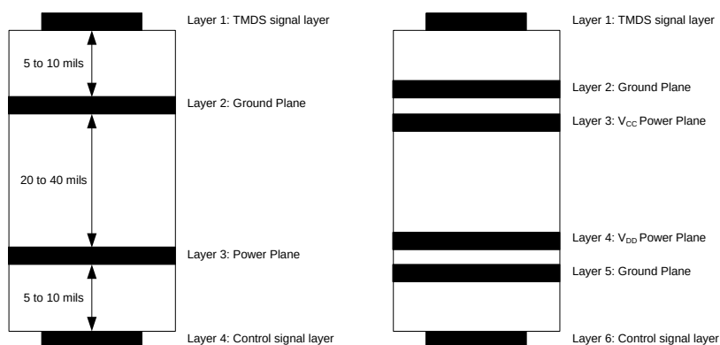
Figure 38. Recommended 4- or 6-Layer PCB Stack
