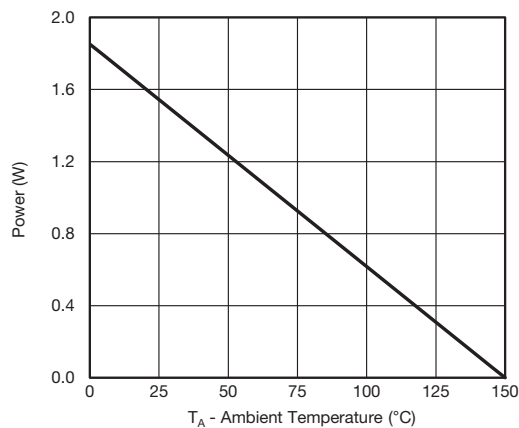
Power, Junction-to-Ambient
