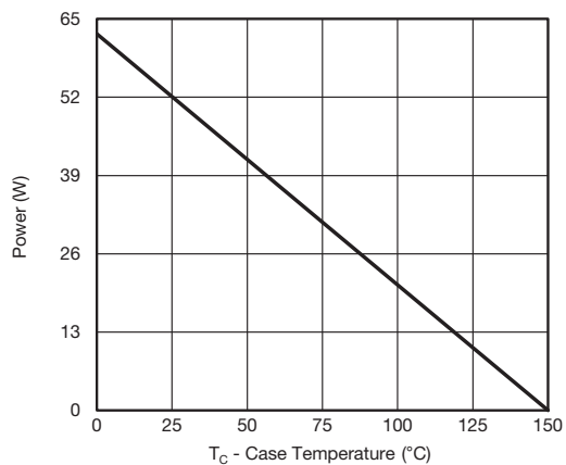
Power, Junction-to-Case
