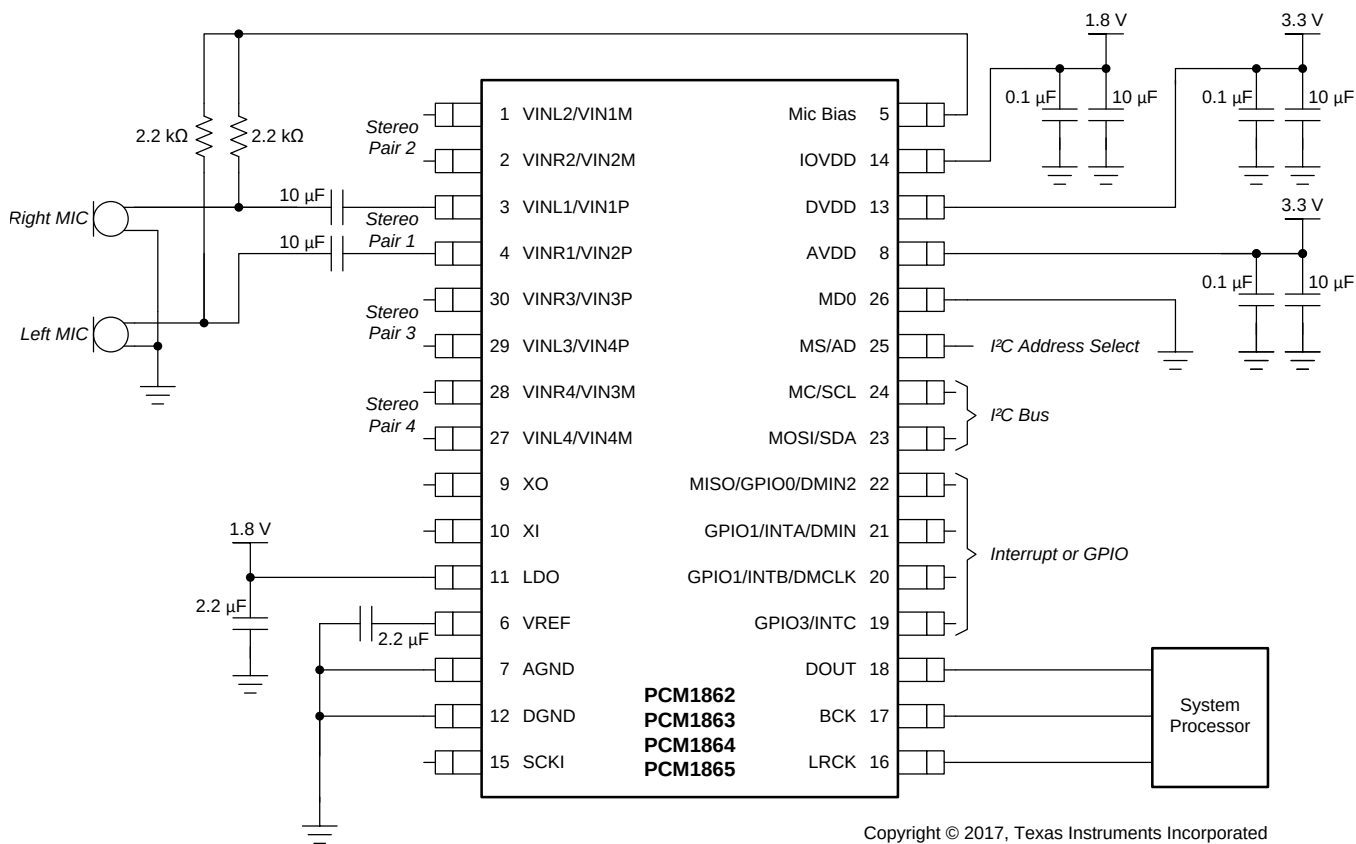
图 66. Stereo Recording Application for PCM186x Software-Controlled Devices in Slave PLL Mode with 1.8-V IOVDD
