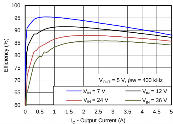
Figure 47. Efficiency vs Load Current
