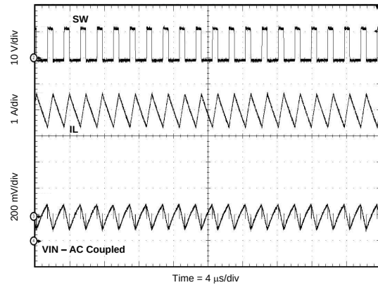
Figure 44. Input Ripple CCM
