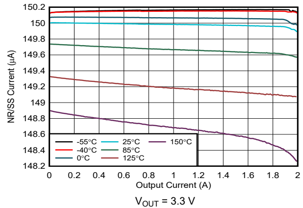
图 6-40. I_{NR/SS} vs I_{OUT} and Temperature for V_{IN} = 3.8\text{ V}
