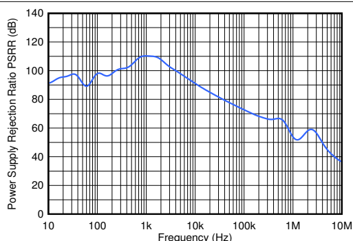
图 8-30. PSRR vs Frequency
