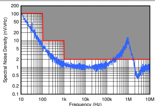
图 8-29. Output Noise vs Frequency
