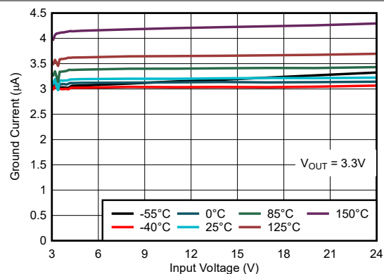
Figure 5-8. Ground Current vs V_{IN}
