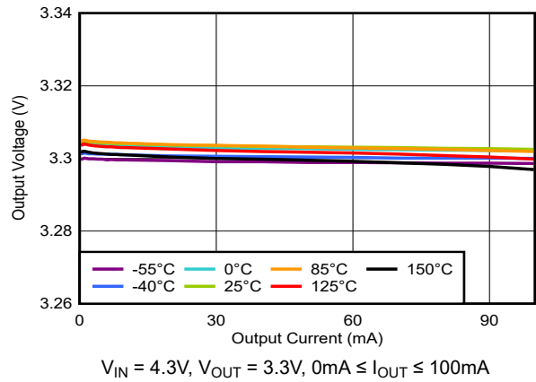
Figure 5-2. Load Regulation
