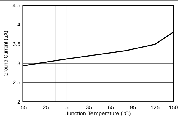
Figure 5-7. Ground Current vs Temperature
