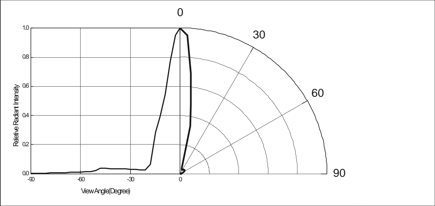
Relative Radiant Intensity vs. Angular Displacement
