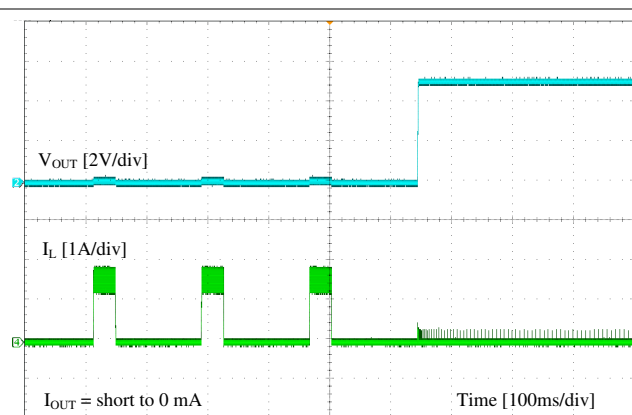
图 8-10. Short Recovery
