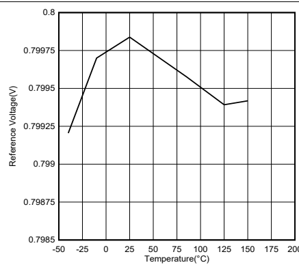
图 6-12. Reference Voltage Versus Temperature
