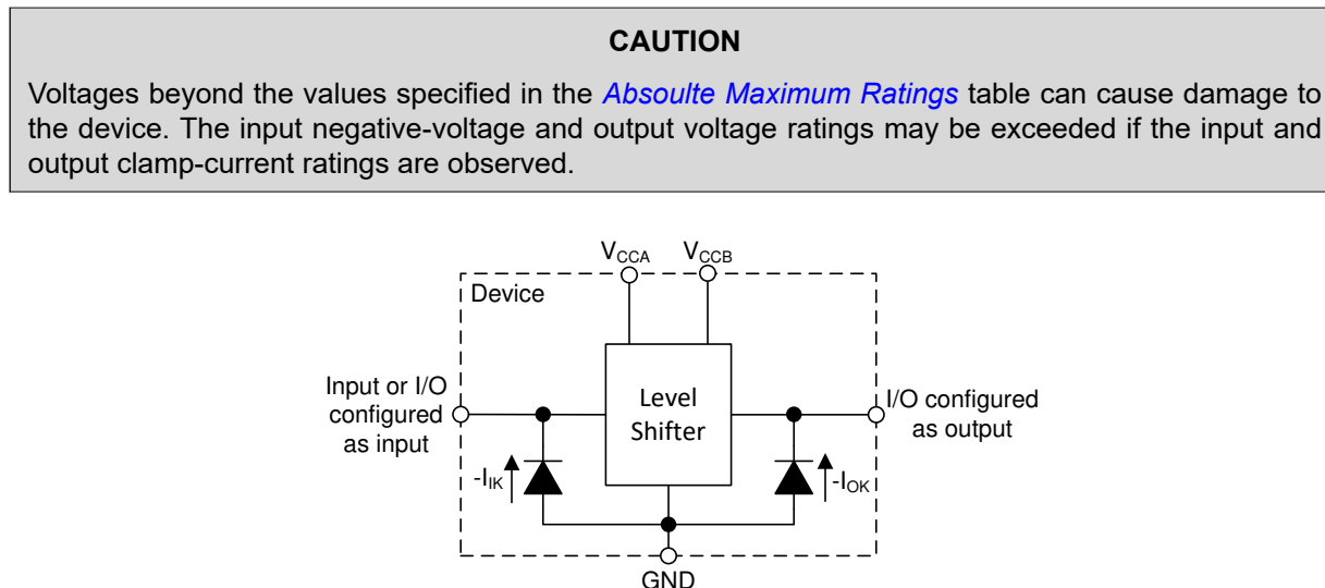
图 9-2. Electrical Placement of Clamping Diodes for Each Input and Output
