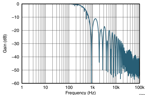
图 7-2. Frequency Response
