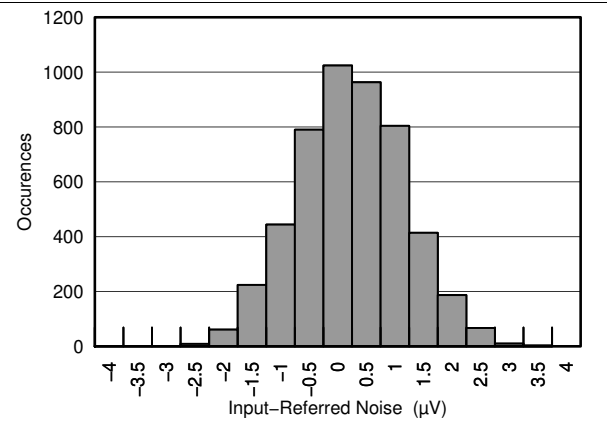
Figure 3. Noise Histogram
