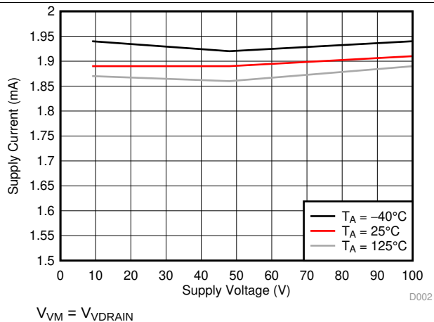
图 3. V_{DRAIN} Supply Current Over Supply Voltage
