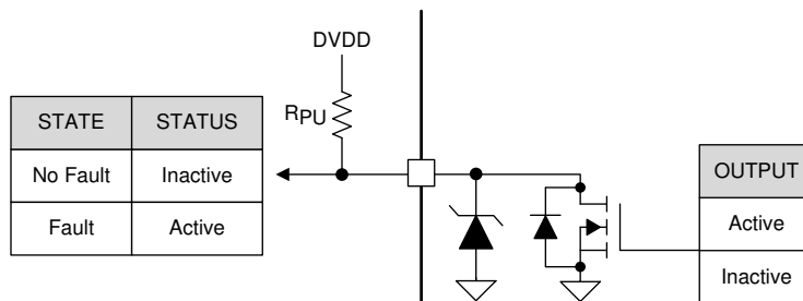
图 40. Open-Drain Output Pin Structure
