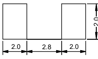
Recommended Pad Size (mm)
