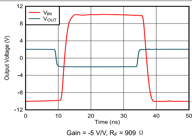
图 7-27. Inverting Large-Signal Transient Response
