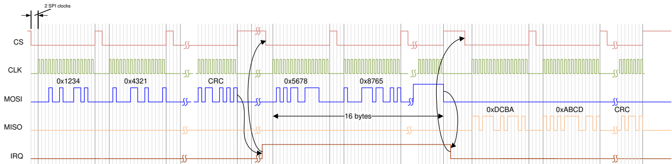
图 8-12. SPI Communication
