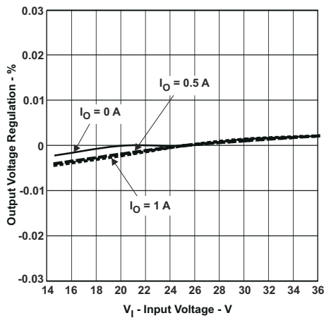
图 7-13. Output Voltage Regulation % vs Input Voltage
