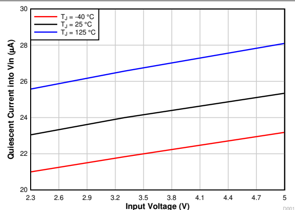
图 6-6. Quiescent Current into V_{IN} vs Input Voltage
