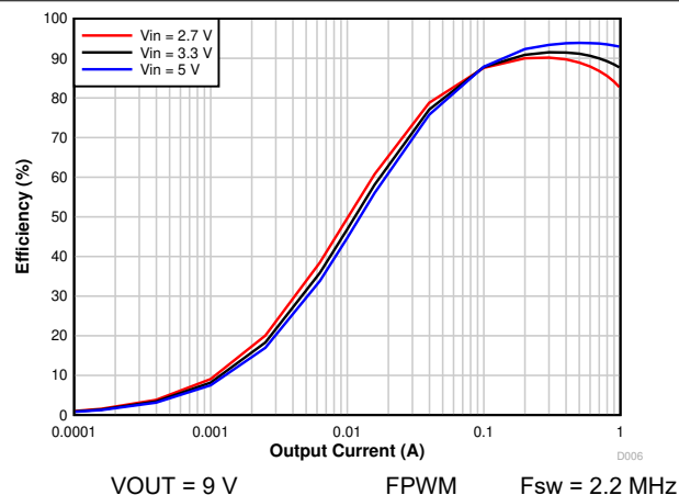
图 6-4. 9 V OUT Efficiency vs Output Current
