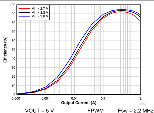
图 6-2. 5 V OUT Efficiency vs Output Current
