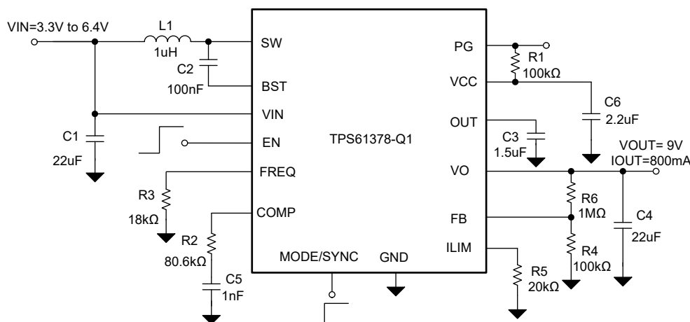
图 8-1. Typical Application
