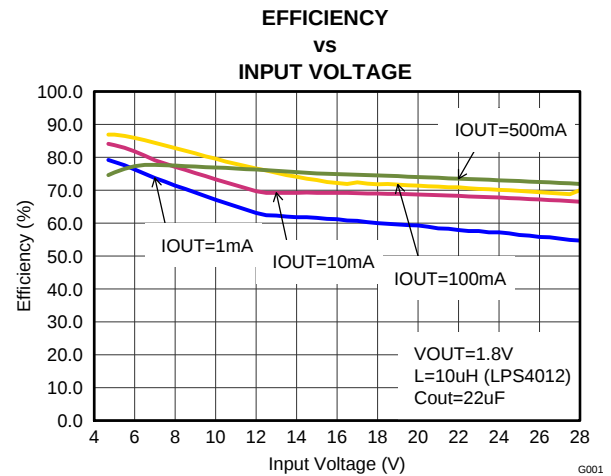
Figure 14. Vout=1.8V
