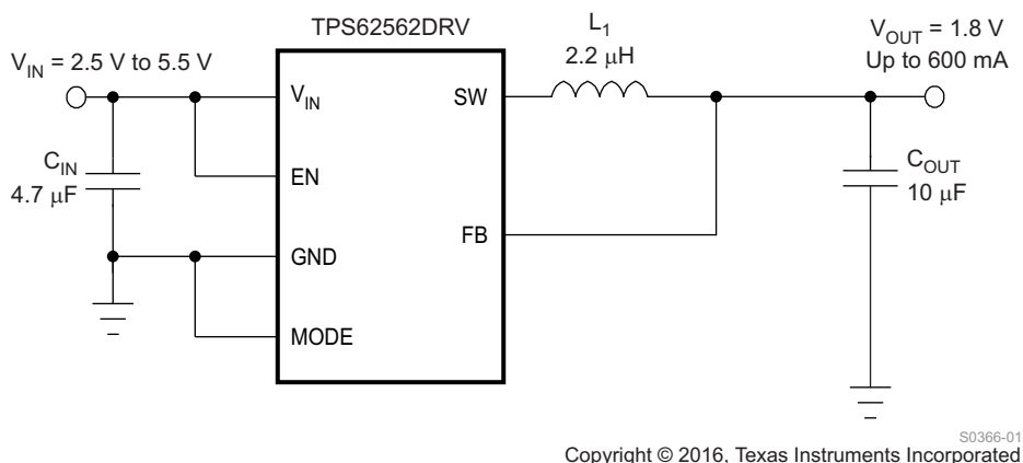
Figure 32. TPS62562 Fixed 1.8-V Output
