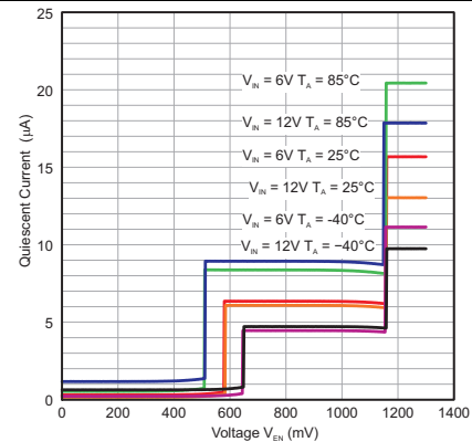
Figure 4. Quiescent Current vs. VEN Voltage, Falling VEN
