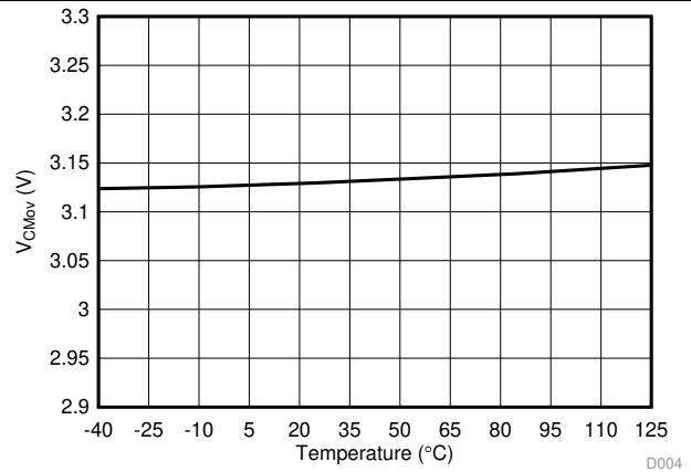
Figure 7. Common-Mode Overvoltage Detection Level vs Temperature
