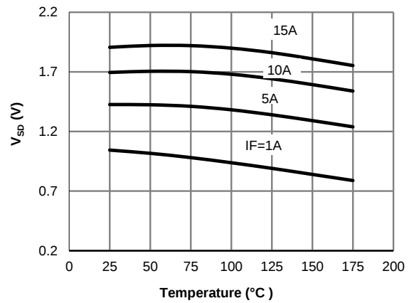
Figure 22: Diode Forward voltage vs. Junction Temperature
