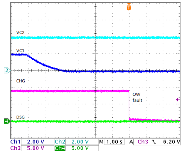
图 10-15. OW Fault Protection, Low Voltage—Open Cell1 Connection
