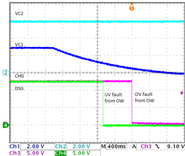
图 10-14. OW Fault Protection—Open Cell1 To PCB Connection
