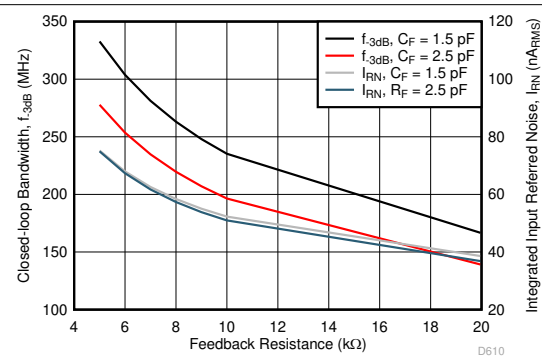
图 10-3. Bandwidth and Noise vs Feedback Resistance
