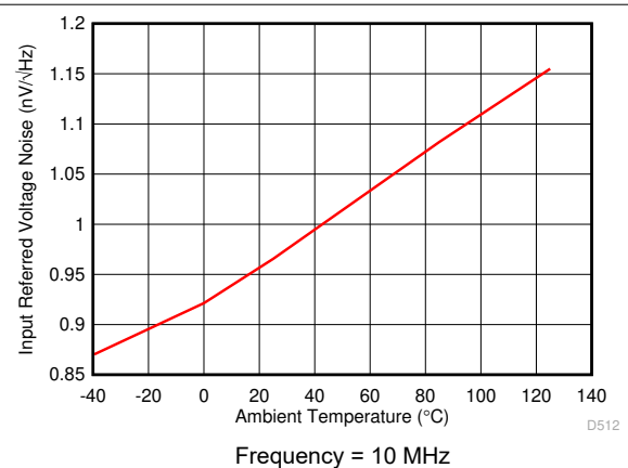
Figure 7-12. Voltage Noise Density vs Ambient Temperature
