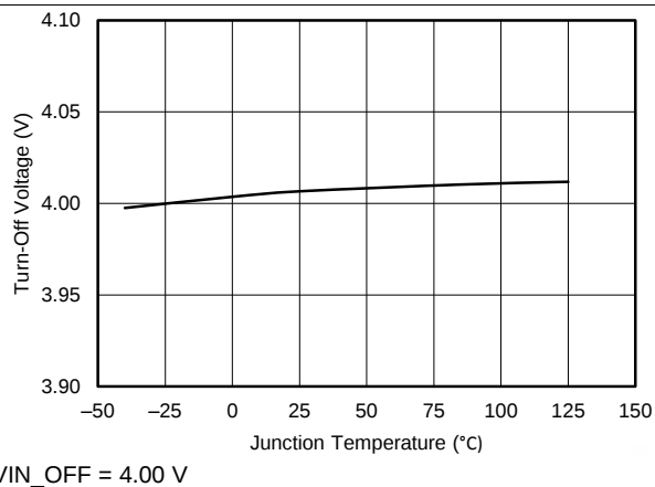
Figure 9. Turn-Off Voltage vs. Junction Temperature
