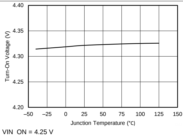
Figure 8. Turn-On Voltage vs. Junction Temperature
