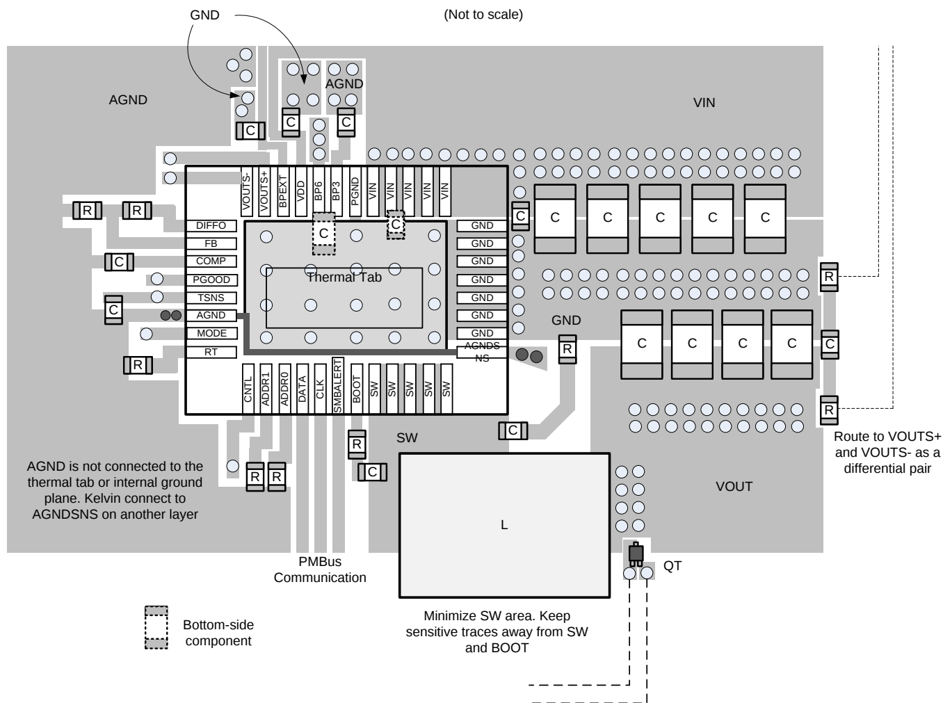
Figure 45. PCB Layout Recommendation
