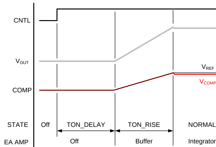
Figure 23. Soft-Start
