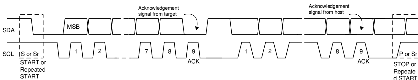
图 9-14. Data Transfer on the I²C Bus
