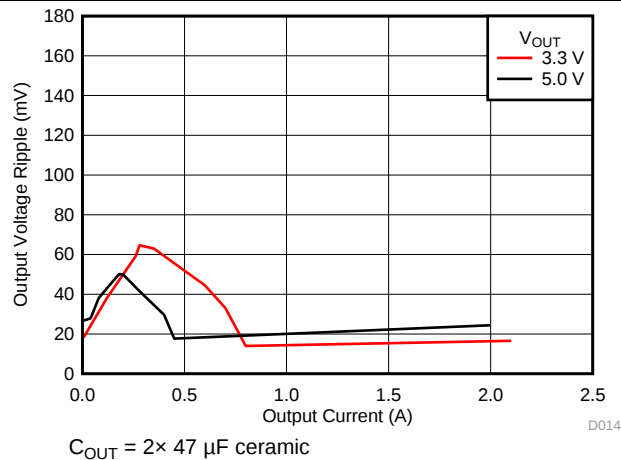
图 14. Voltage Ripple vs Output Current
