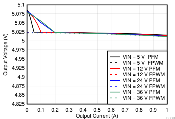
图 8-10. Line and Load Regulation
