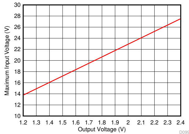
图 8-3. Maximum Input Voltage for V_{OUT} < 2.5 V
