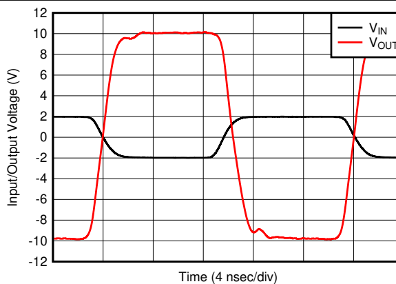
图 8-26. G = -5 V/V Pulse Response
