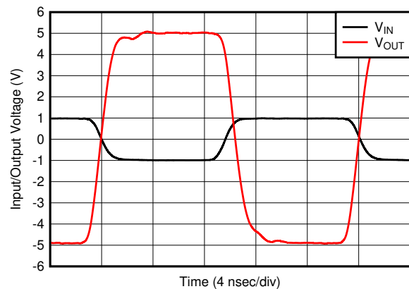
图 8-55. G = 5 V/V Pulse Response
