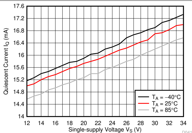
图 8-30. Quiescent Current vs Supply Voltage
