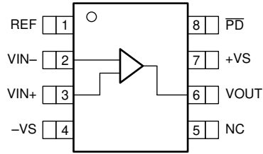
图 6-1. DDA Package, 8-Pin HSOIC With PowerPAD (Top View)
