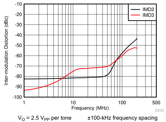
图 8-51. Intermodulation Distortion vs Frequency
