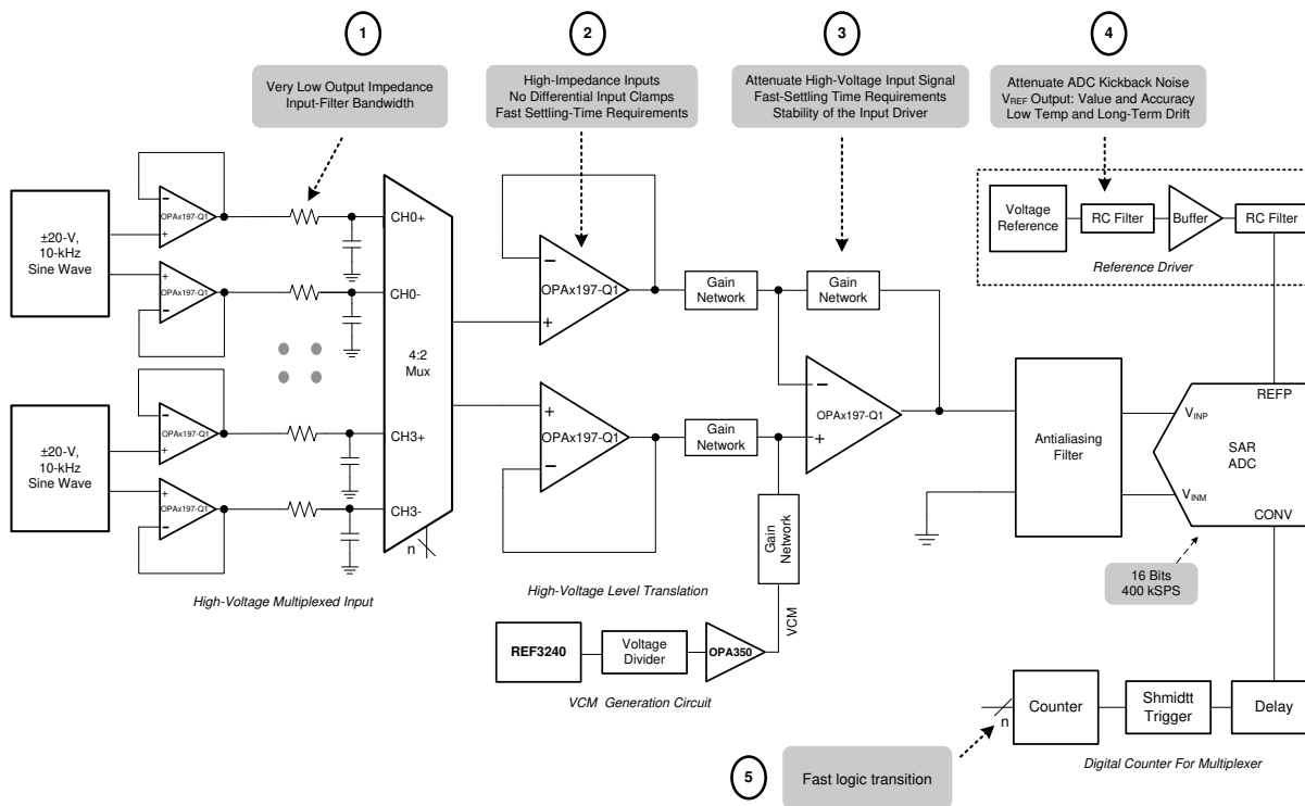
图 8-1. OPAx197-Q1 in 16-Bit, 400-kSPS, 4-Channel, Multiplexed Data Acquisition System for High-Voltage Inputs With Lowest Distortion
