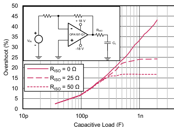
图 7-7. Small-Signal Overshoot vs Capacitive Load (100-mV Output Step)
