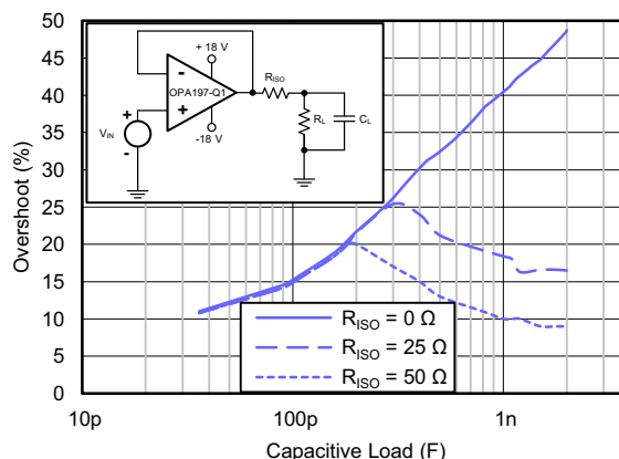
图 7-8. Small-Signal Overshoot vs Capacitive Load (100-mV Output Step)
