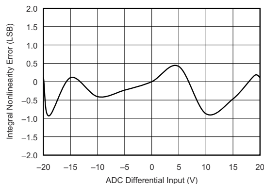
图 8-2. ADC 16-Bit Linearity Error for the Multiplexed Data Acquisition Block
