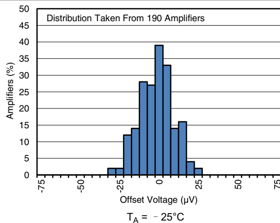
图 6-5. Offset Voltage Production Distribution at -25°C
