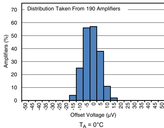
图 6-4. Offset Voltage Production Distribution at 0°C
