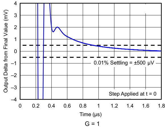
图 6-41. Settling Time (5-V Negative Step)
