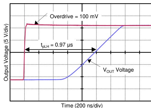
图 6-44. Propagation Delay Rising Edge
