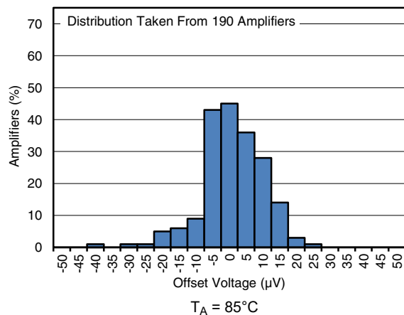
图 6-3. Offset Voltage Production Distribution at 85°C
