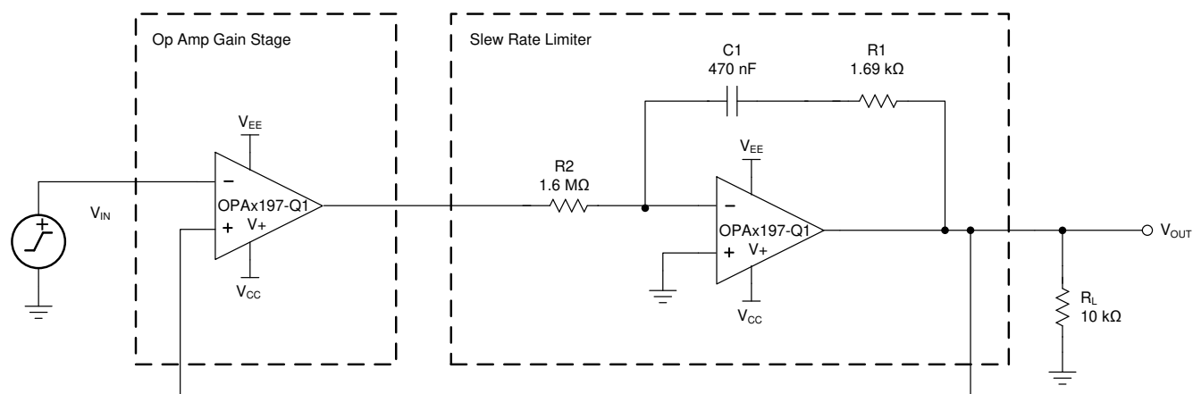
图 8-3. Slew-Rate Limiter Uses One Op Amp
