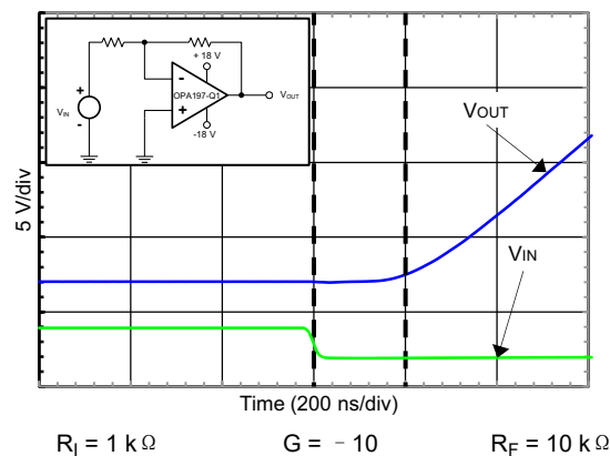
图 6-34. Negative Overload Recovery
