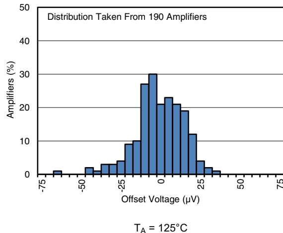
图 6-2. Offset Voltage Production Distribution at 125°C
