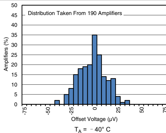
图 6-6. Offset Voltage Production Distribution at -40°C
