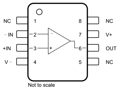
图 5-1. OPA197-Q1 DGK Package, 8-Pin VSSOP, Top View
