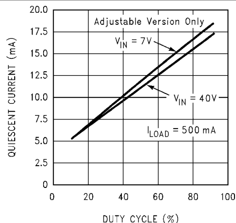
图 6-14. Quiescent Current vs Duty Cycle
