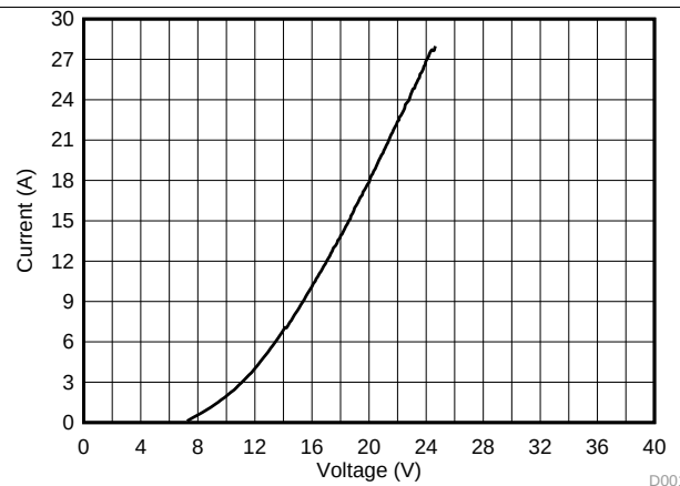
Figure 3. Clamping Voltage V_{TLP} = F(I_{TLP}) , PIN1 to PIN2
