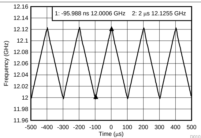
Figure 10. VCO Ramping 12-GHz to 12.125-GHz Calibration Free
