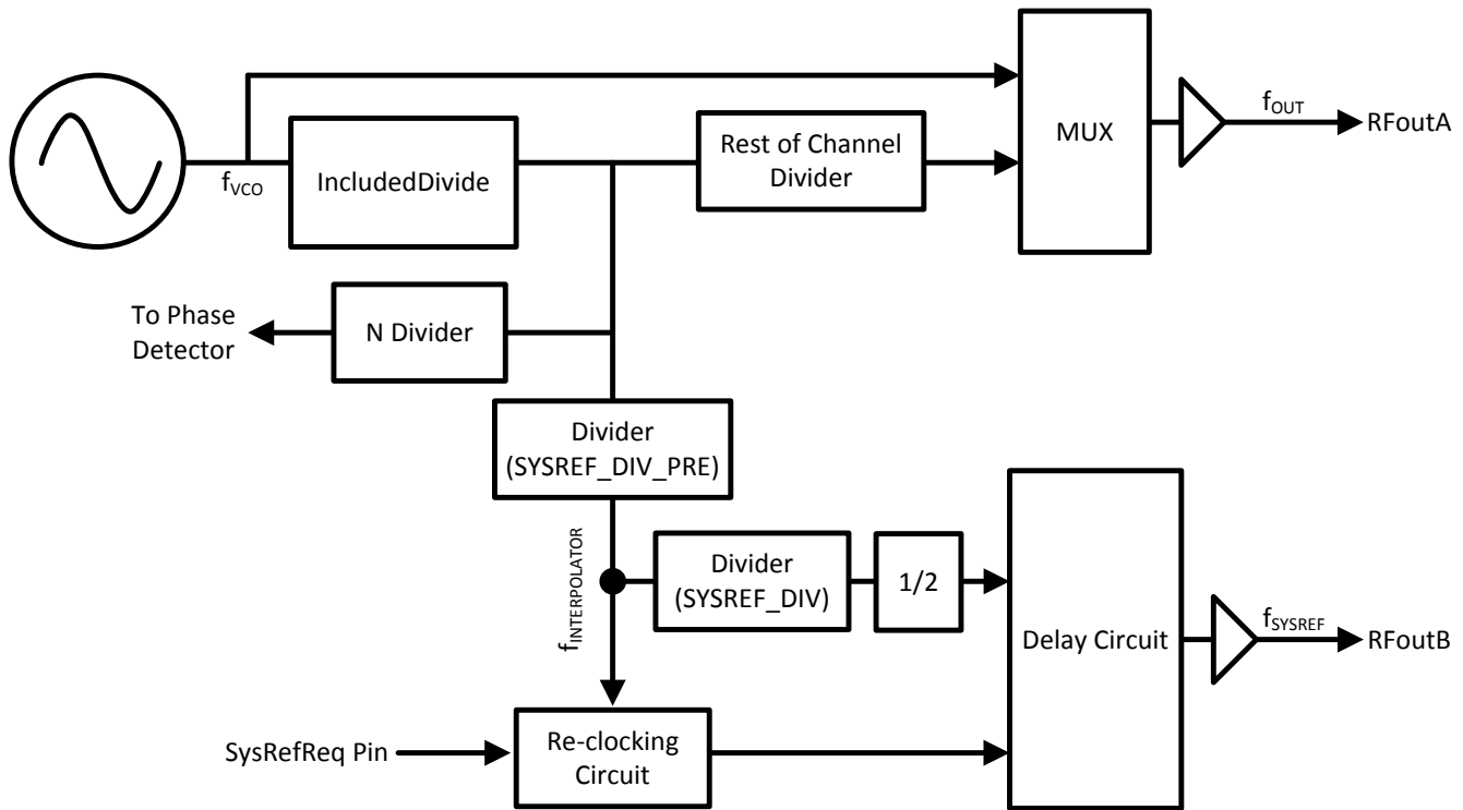
Figure 30. SYSREF Setup
