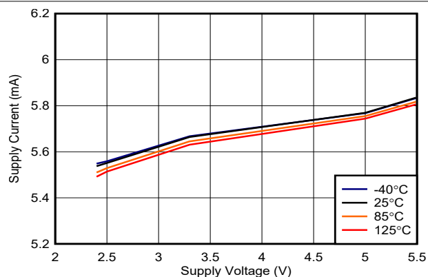
图 6-36. TLV3603 Supply Current vs. Voltage (Output High)
