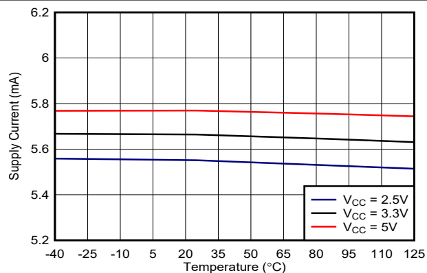
图 6-38. TLV3603 Supply Current vs. Temp (Output High)
