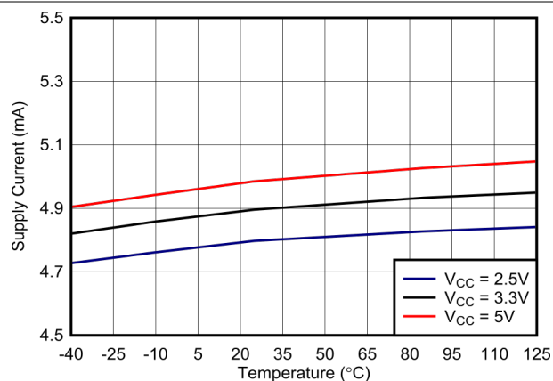
图 6-34. TLV3601 Supply Current vs. Temp (Output High)
