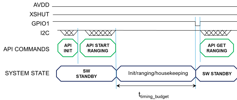
Figure 8. Ranging sequence
