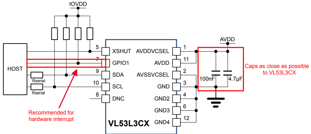
Figure 3. VL53L3CX schematic
