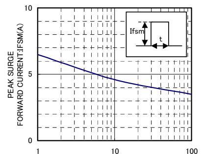
IFSM-t CHARACTERISTICS
