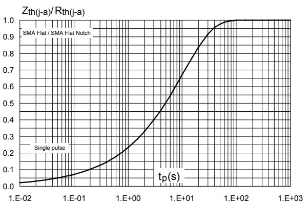
Figure 8. Relative variation of thermal impedance junction to ambient versus pulse duration (SMA Flat)
