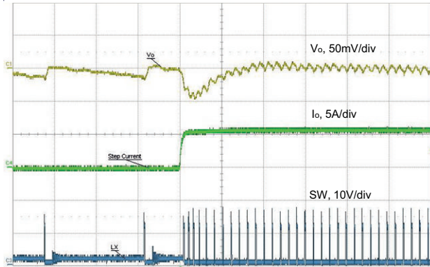
Fig. 50 - Load Step, 0.1 A to 6 A, 1 A/ \mu s, t = 10\text{ }\mu s/div Skip Mode Enabled
